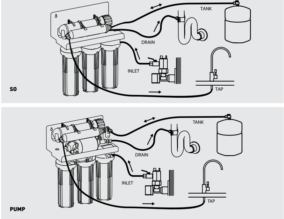
Hydraulic connections diagram
